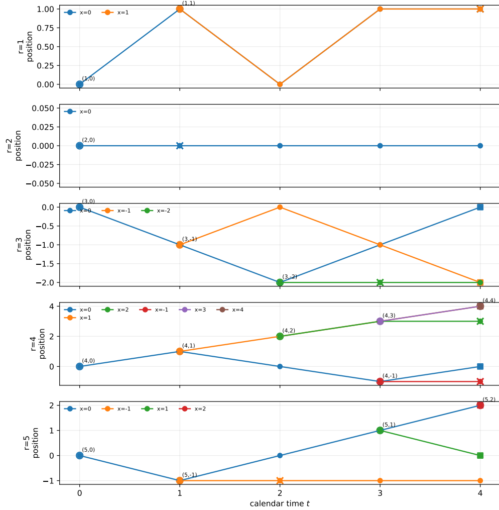
FIGURE 1. Labeled particle trajectories through the finite horizon.
