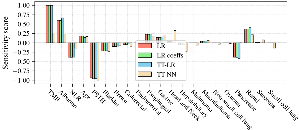
Feature sensitivity with LR coefficients
