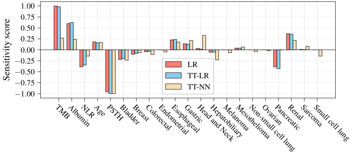
Feature sensitivity
