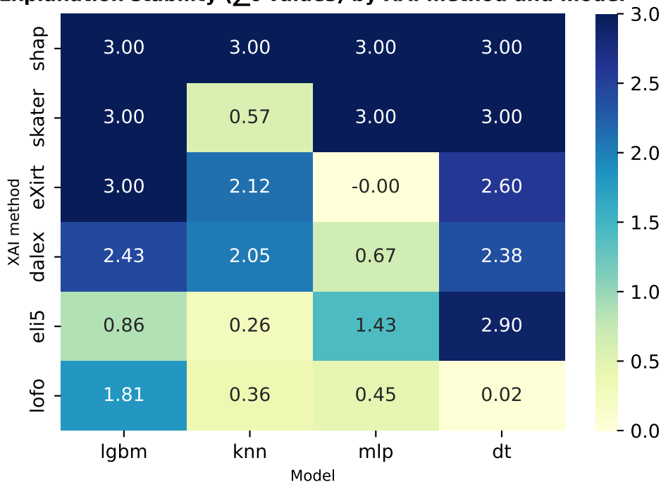
Explanation stability ( \sum_C values) by XAI method and model
