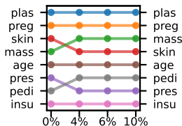
(J) EXIRT | KNN ( \sum_C : 2.12)
