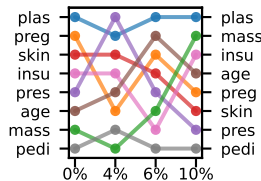
(X) LOFO | DT ( \sum_C : 0.02)
