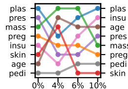
(W) LOFO | MLP ( \sum_C : 0.45)
