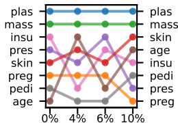
(V) LOFO | KNN ( \sum_C : 0.36)
