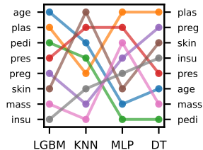
(F) LOFO | Model Dependence ARD: 8.692
