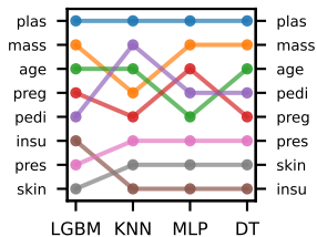
(B) SHAP | Model Dependence ARD: 3.588
