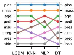
(A) DALEX | Model Dependence ARD: 3.133
