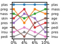
(S) ELI5 | MLP (ARD: 4.344)
