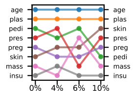
(U) LOFO | LGBM (ARD: 3.721)
