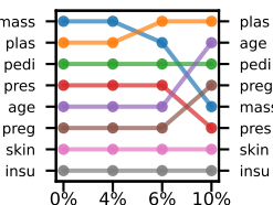
(T) ELI5 | DT (ARD: 0.471)
