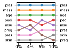
(M) EXIRT | LGBM (ARD: 0.0)
