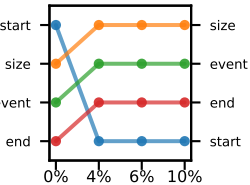
(T) DALEX | DT (ARD: 1.971)
