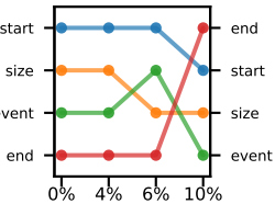
(X) LOFO | DT (ARD: 1.626)
