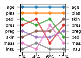
(U) LOFO | LGBM (ARD: 3.721)
