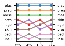
(U) LOFO | LGBM (ARD: 3.721)
