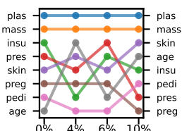
(V) LOFO | KNN (ARD: 5.531)
