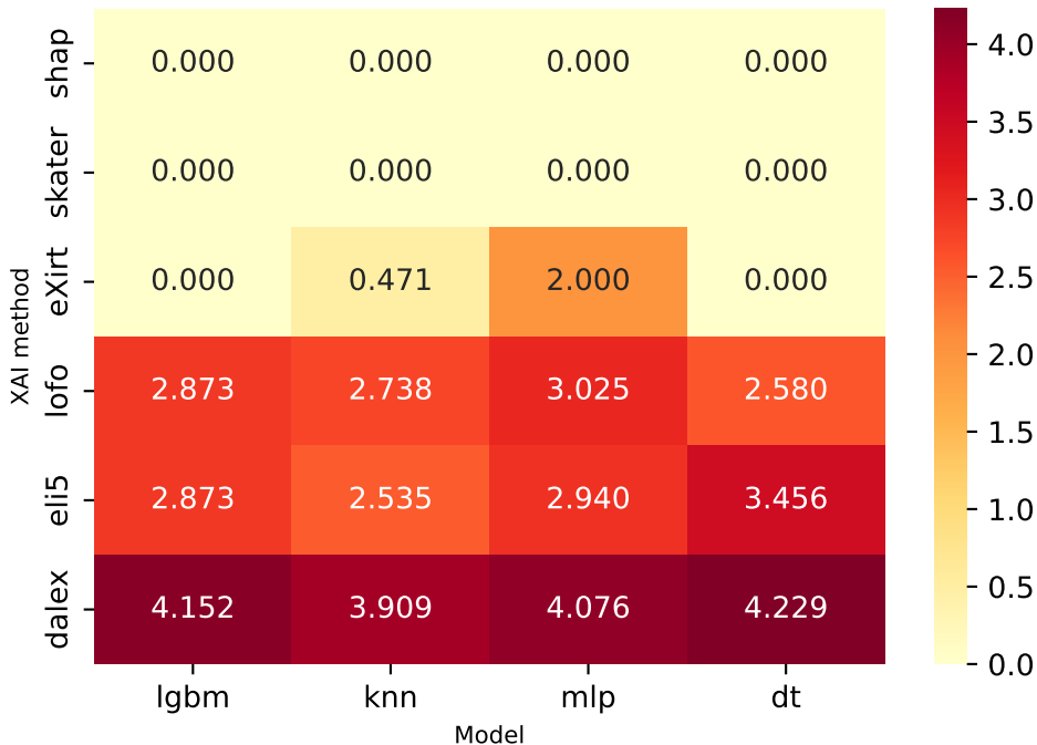
Explanation Volatility (ARD values)
