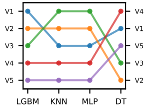
(F) ELI5 | Model Dependence ARD: 3.519
