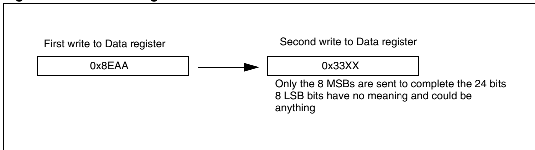
Figure 214. Transmitting 0x8EAA33
