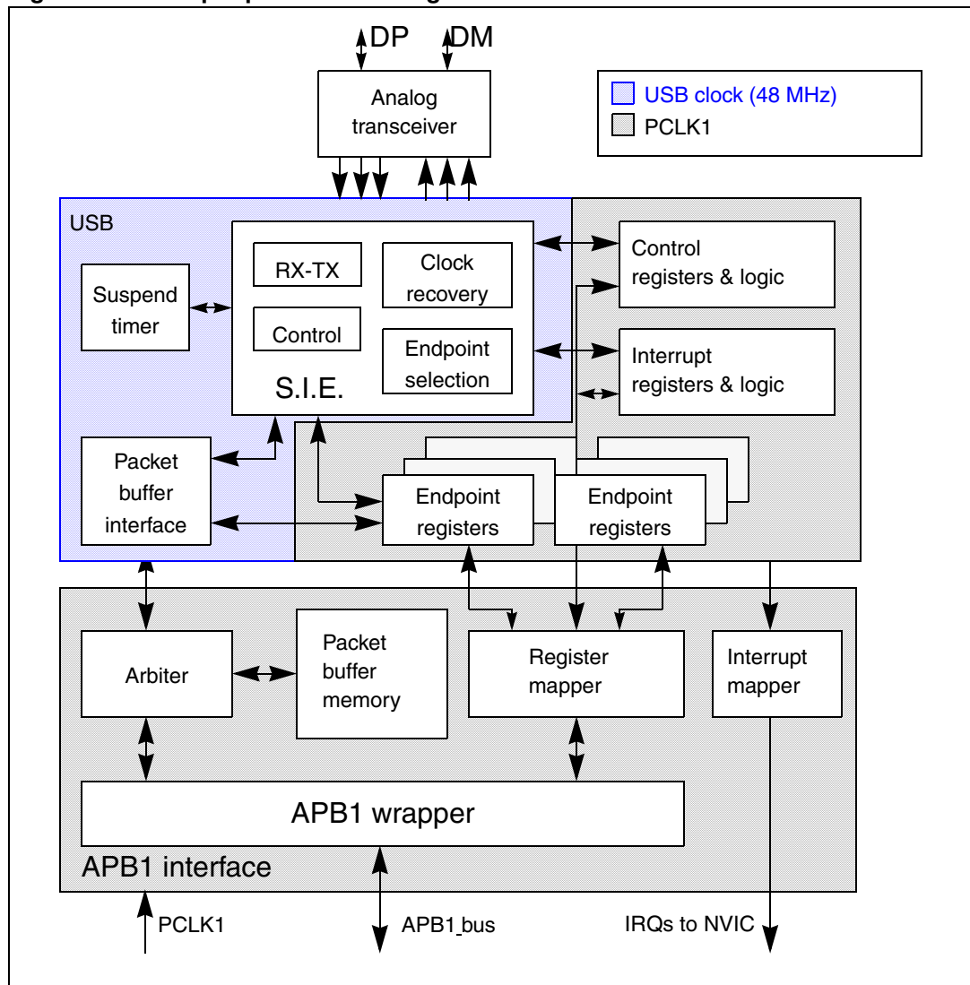
Figure 190. USB peripheral block diagram
