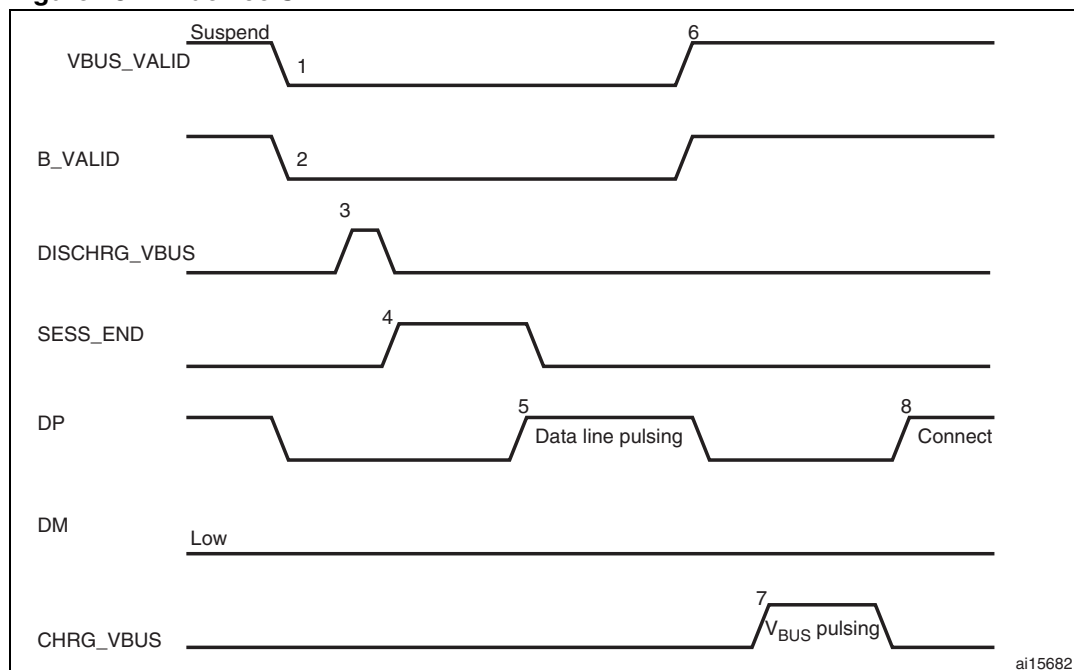
Figure 281. B-device SRP
