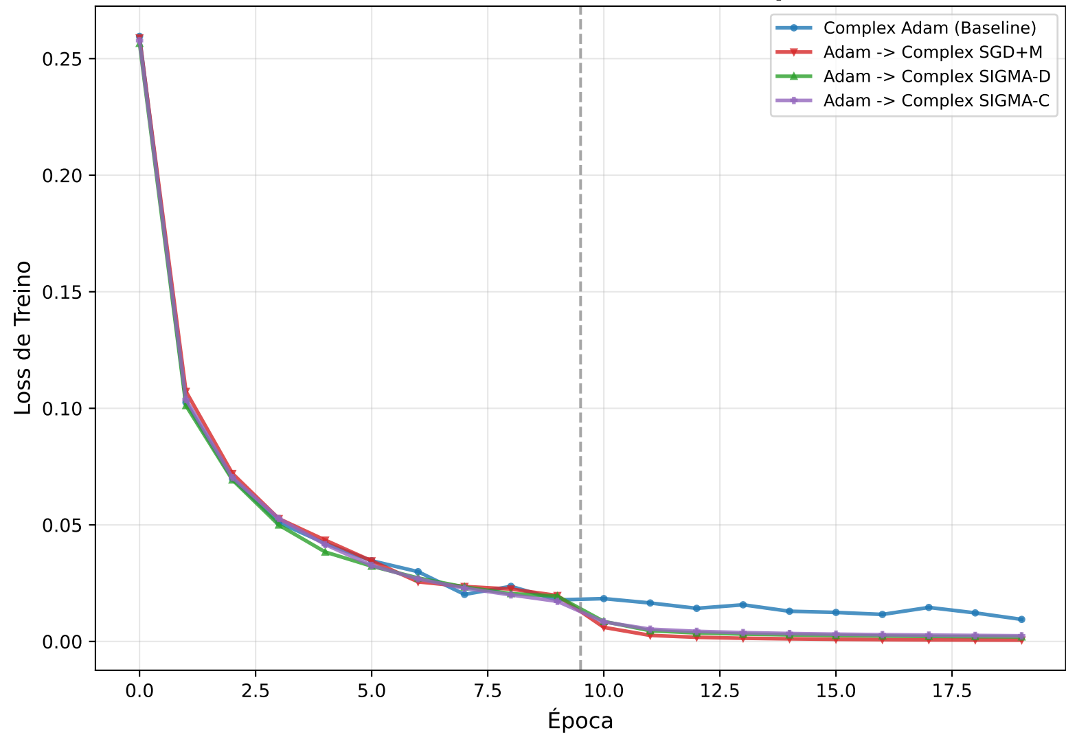
Loss de Treino (Rede Neural Complexa)
