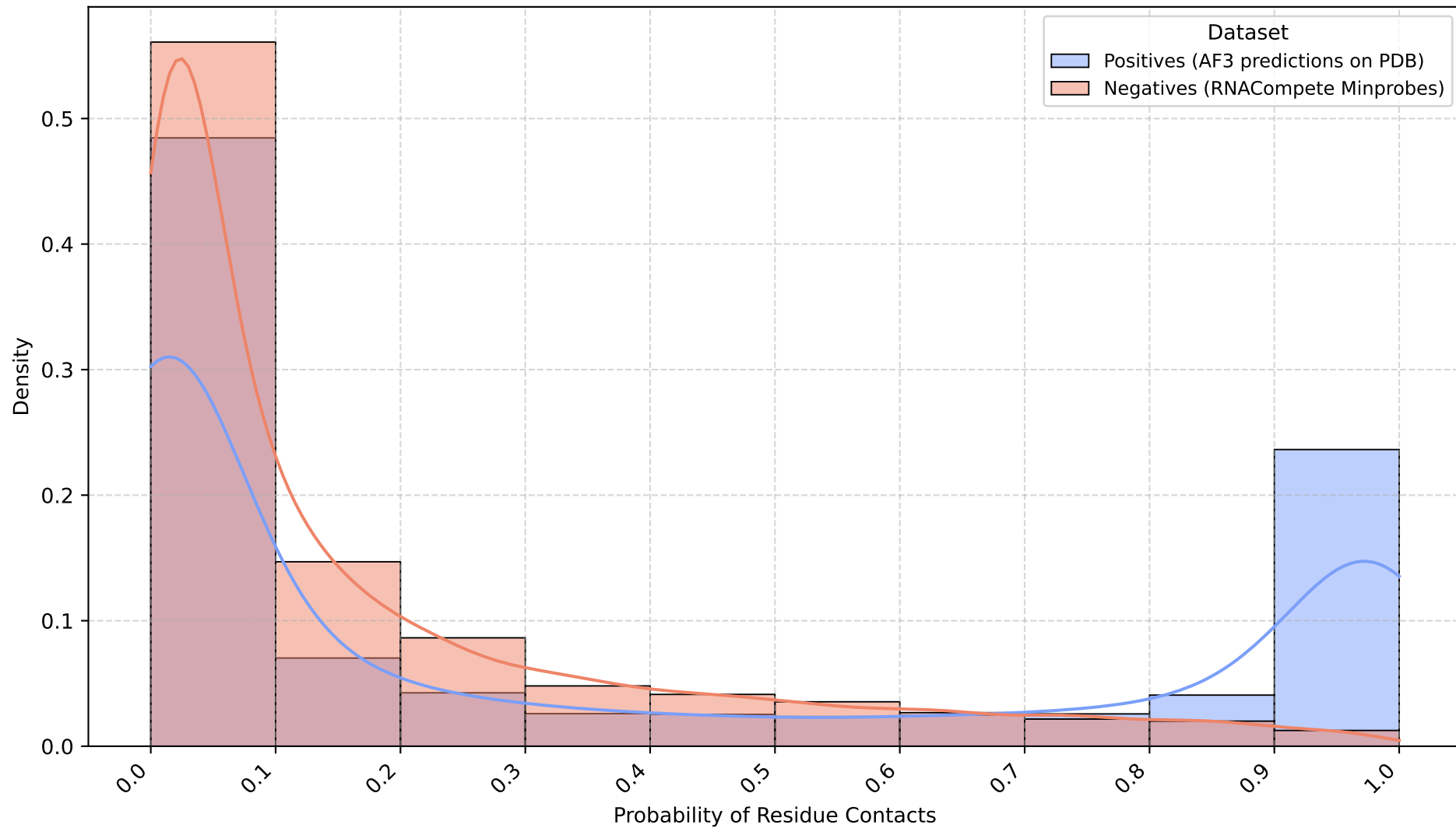
Probability Distribution of Residue Contacts in alternative dataset (Positives vs Negatives)
