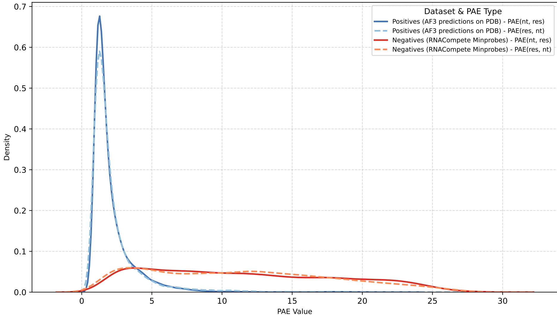
Density Comparison of PAE(nt, res) vs PAE(res, nt) in alternative dataset
