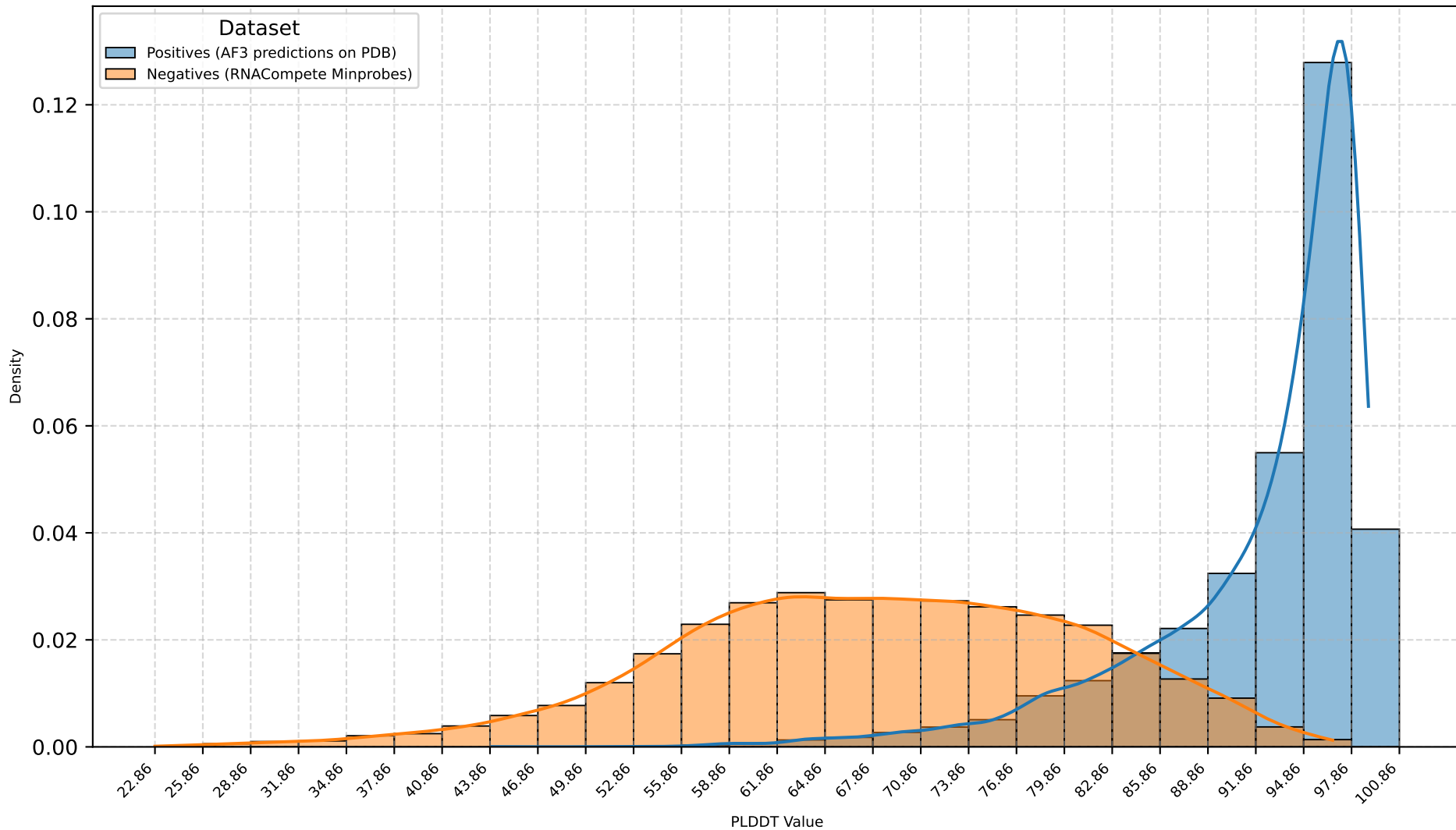
Density Comparison of PLDDT in alternative dataset (Positives vs Negatives)
