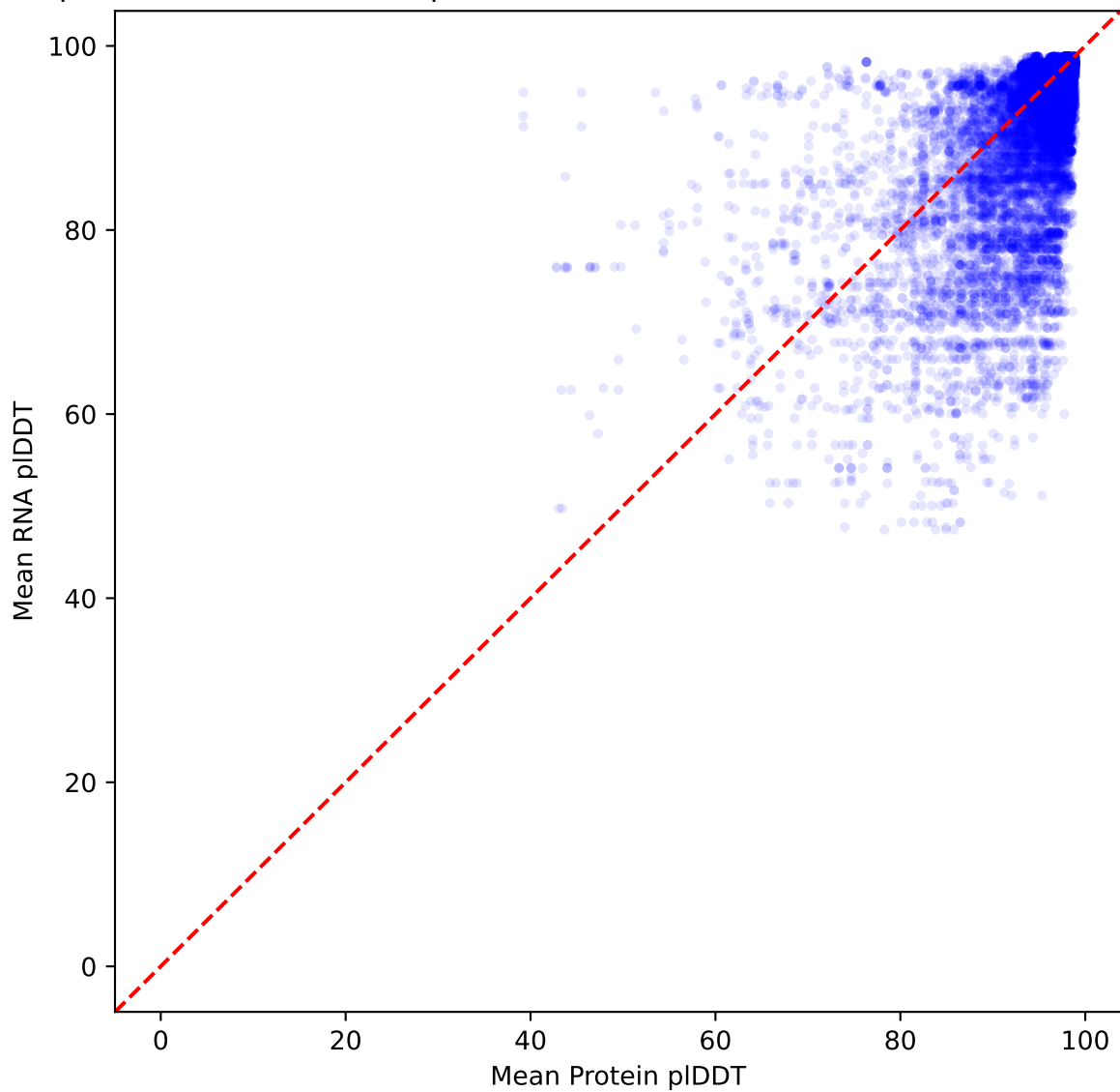
Mean RNA pLDDT vs. Mean Protein pLDDT (Per 3-mer Pair) - alternative dataset (Positives)
