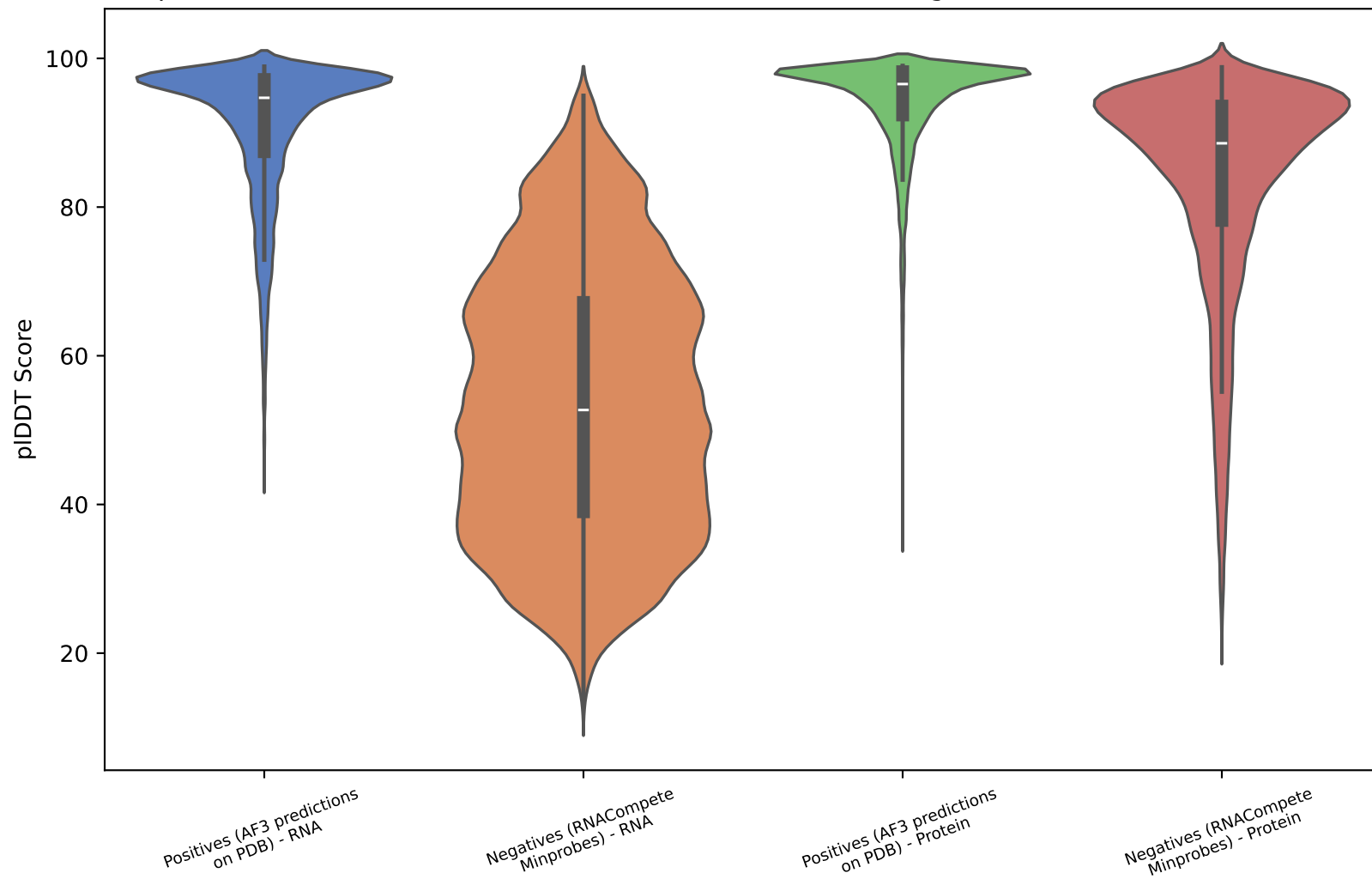
pLDDT Distributions for RNA and Protein (Positives vs Negatives) - alternative dataset
