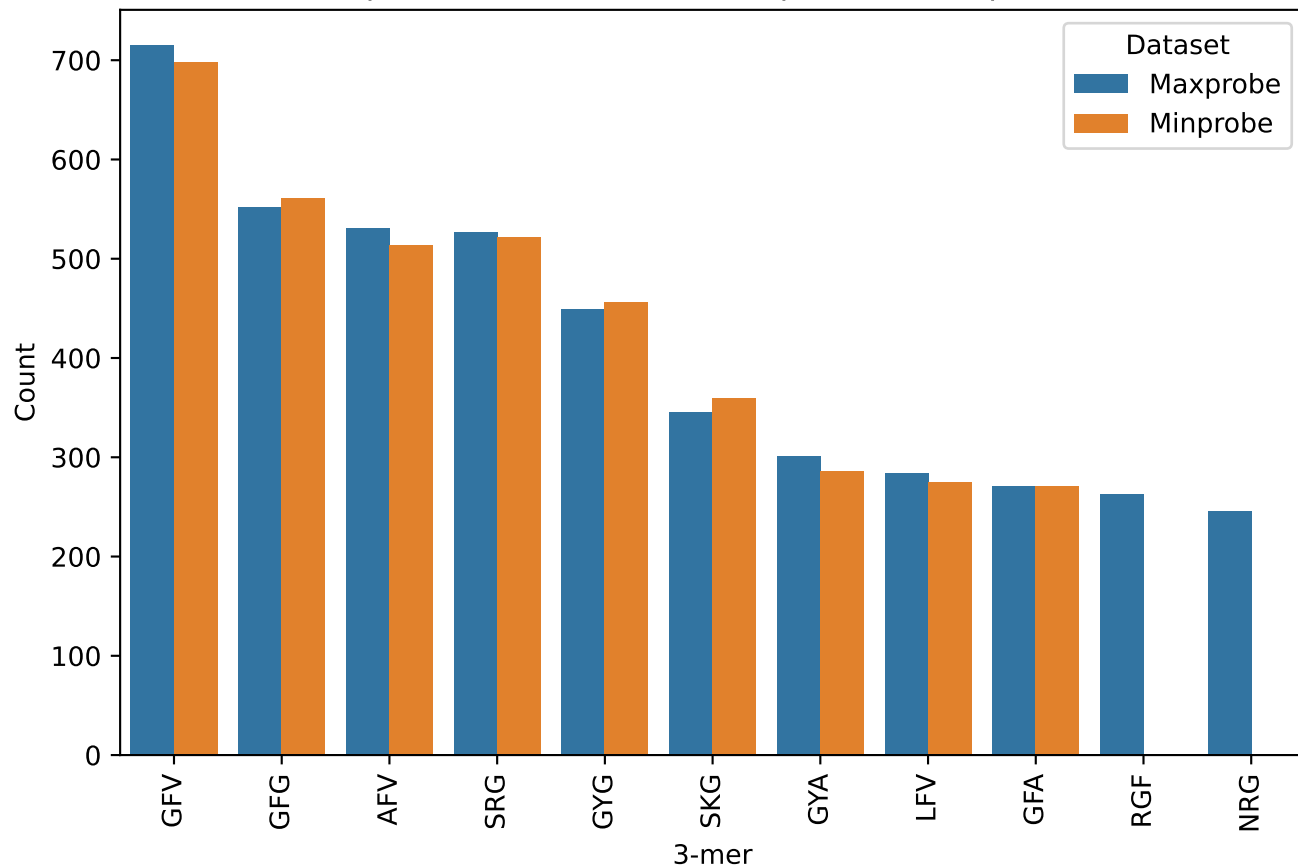
Top 3-mers in Proteins (maxprobe vs minprobe)
