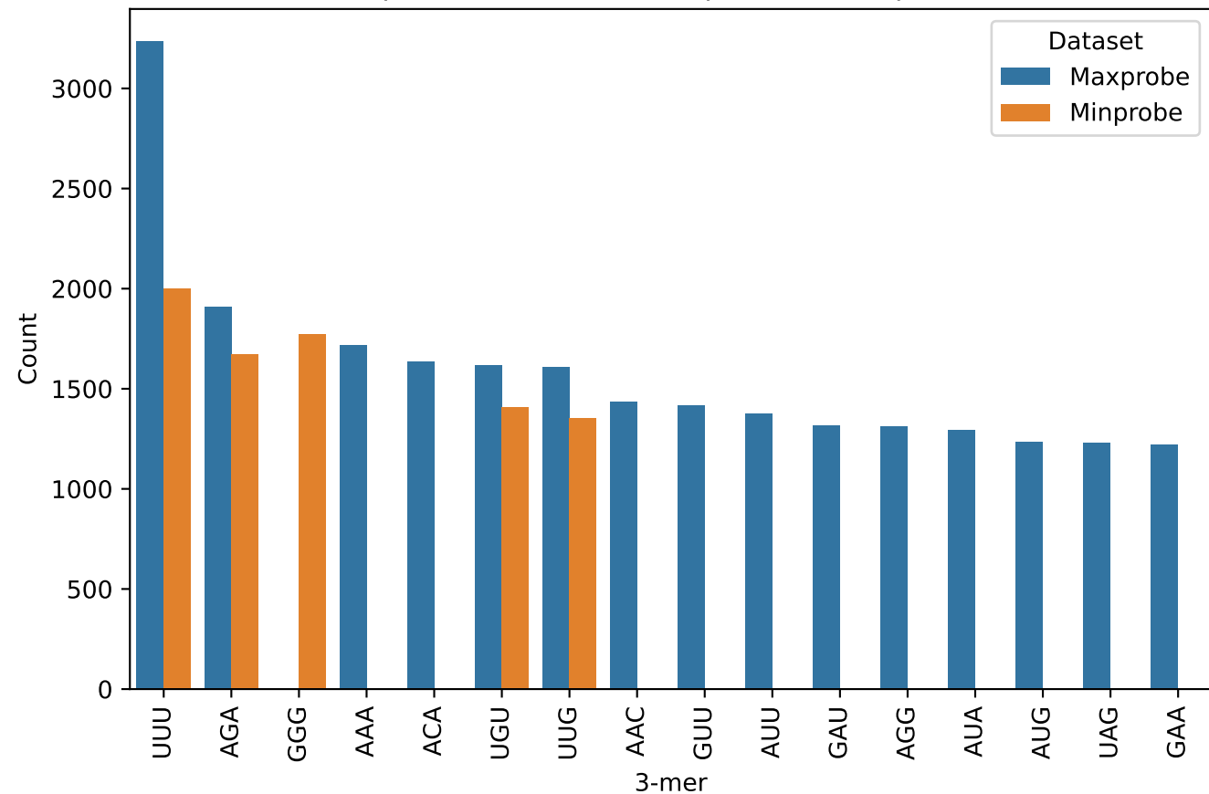
Top 3-mers in RNA (maxprobe vs minprobe)
