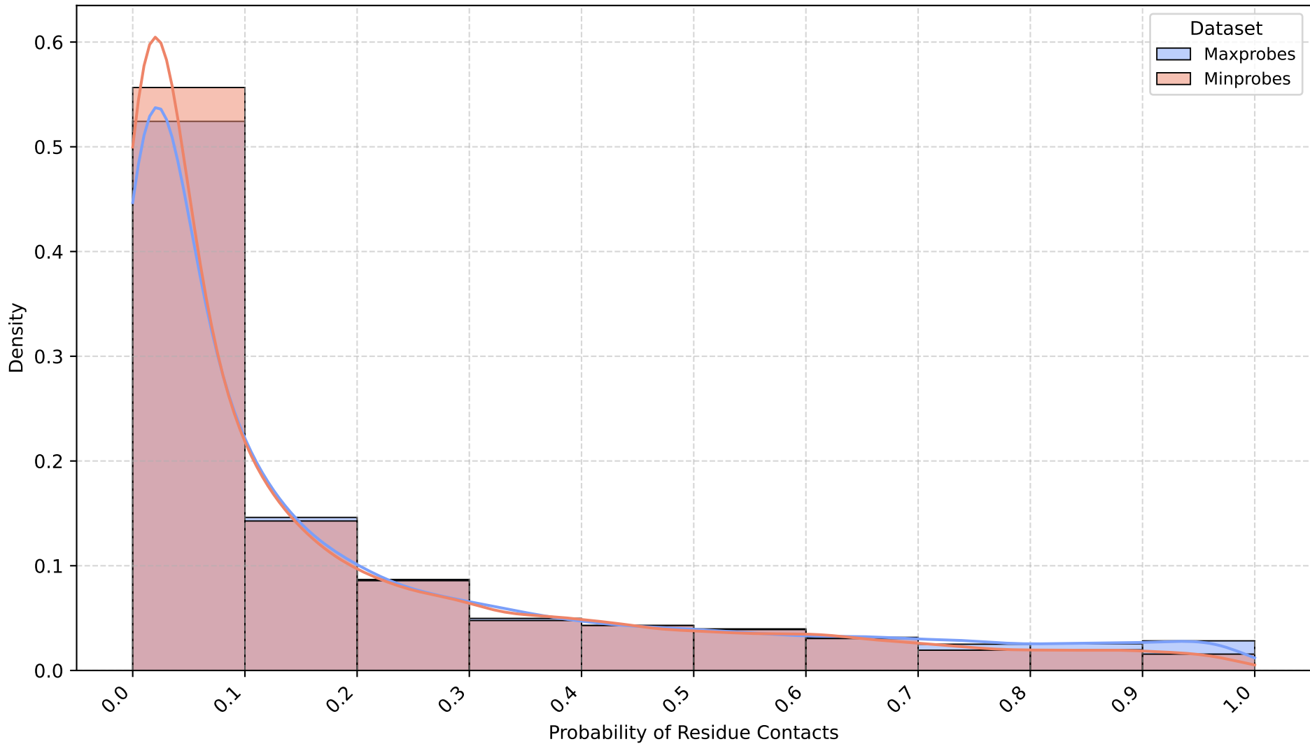
Probability Distribution of Residue Contacts in Augmented RNACompete (Maxprobes vs Minprobes)
