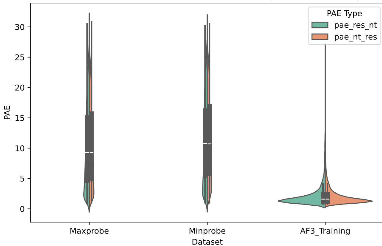
PAE(res, nt) vs. PAE(nt, res) Across Datasets - Augmented RNACompete
