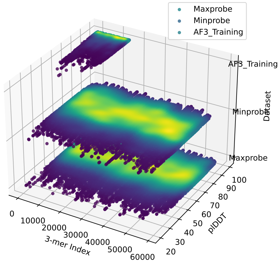
3D KDE Density Plot: 3-mer Frequency vs. pLDDT
