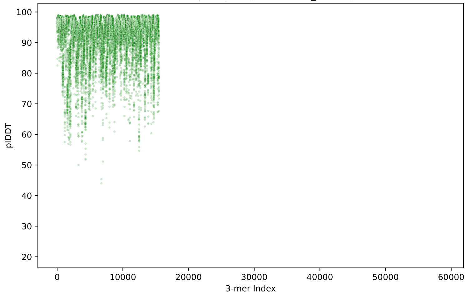
3-mer Frequency vs. pIDDT - AF3_Training
