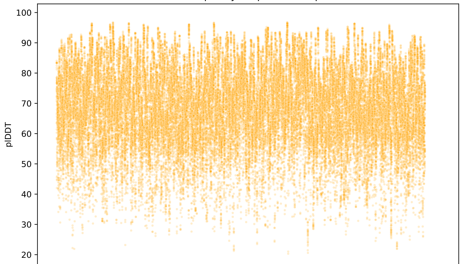
3-mer Frequency vs. pIDDT - AF3_Training
