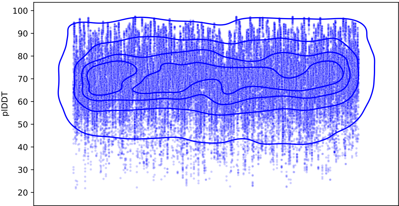
3-mer Frequency vs. pLDDT - Maxprobe
