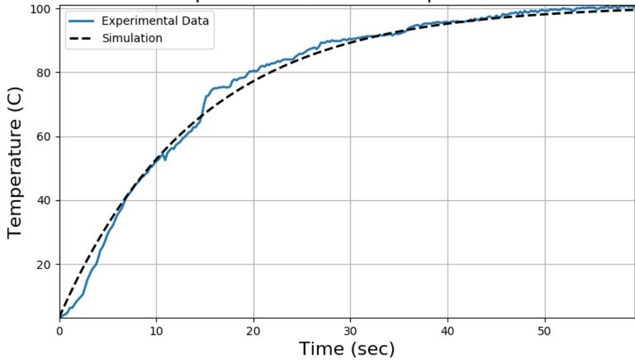
Response of a Thermocouple: odeint
