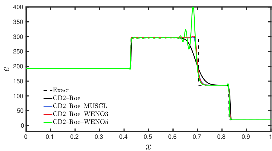
Figure 72: 400 Grid Points
