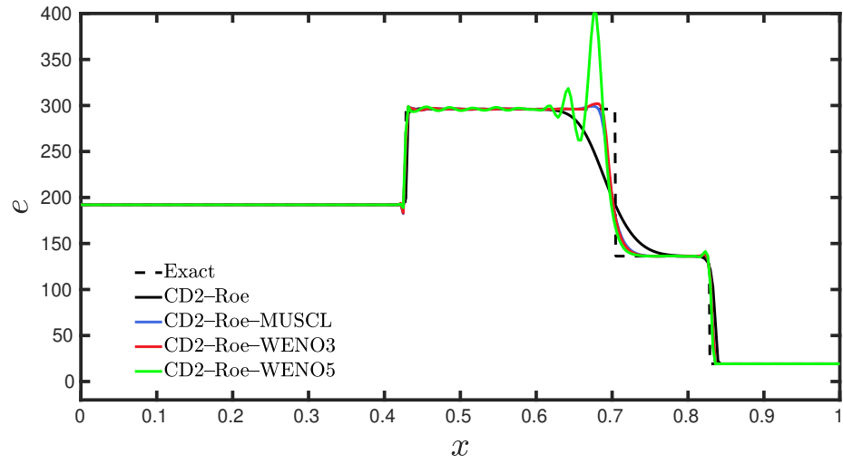
Figure 56: 300 Grid Points
