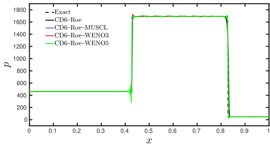
Figure 95: 500 Grid Points
