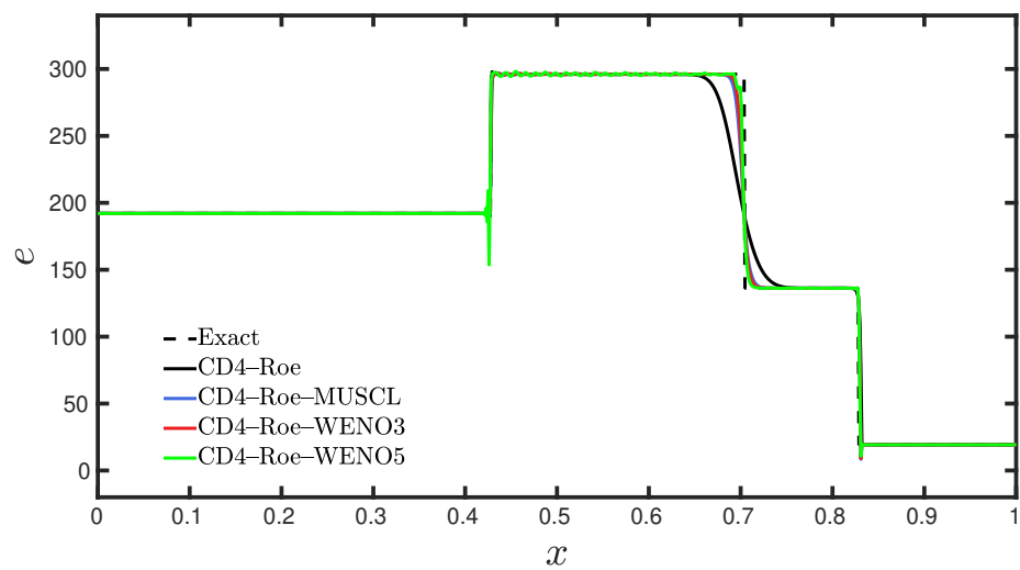
Figure 156: 900 Grid Points
