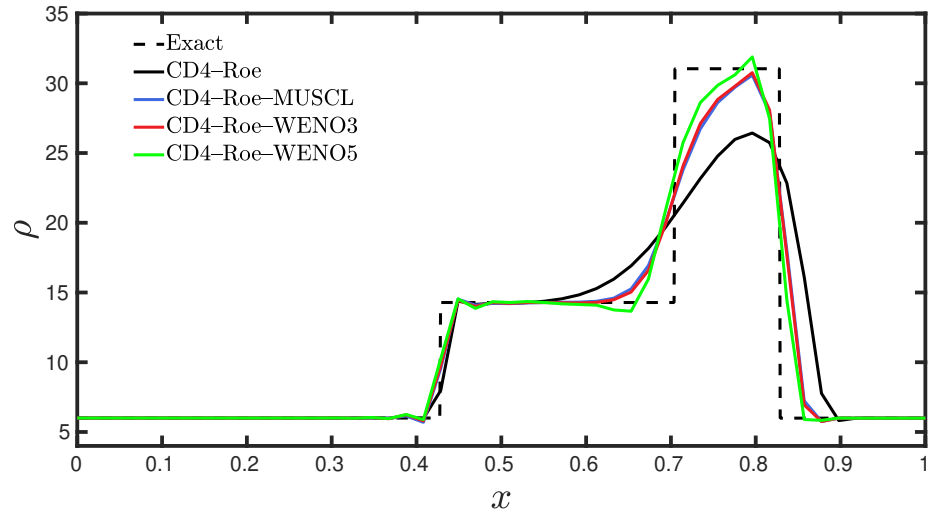
Figure 9: 50 Grid Points
