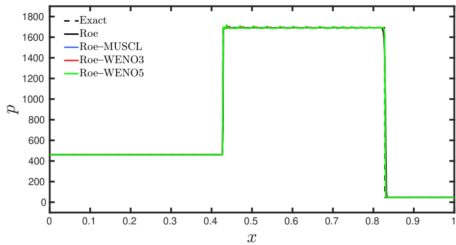
Figure 131: 800 Grid Points
