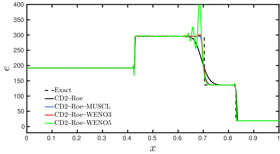
Figure 88: 500 Grid Points
