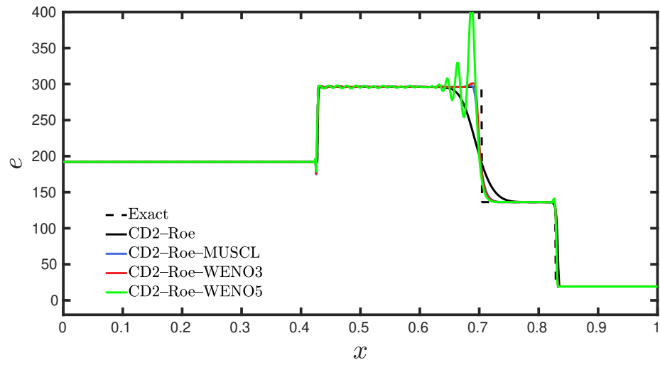
Figure 104: 600 Grid Points
