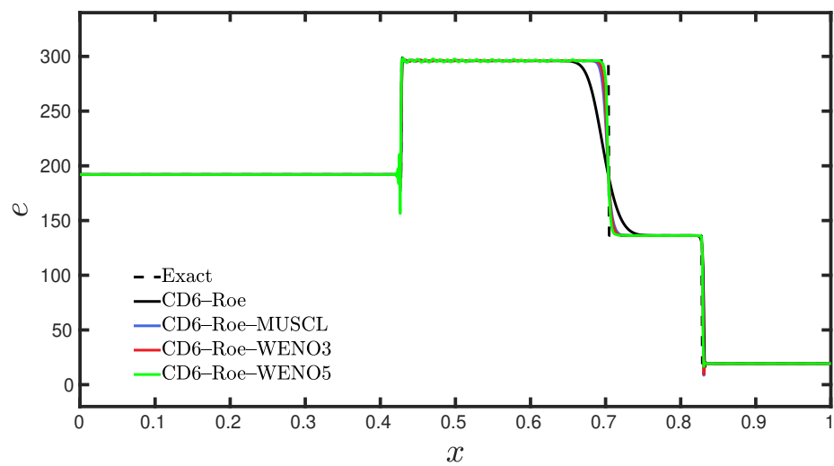
Figure 176: 1000 Grid Points
