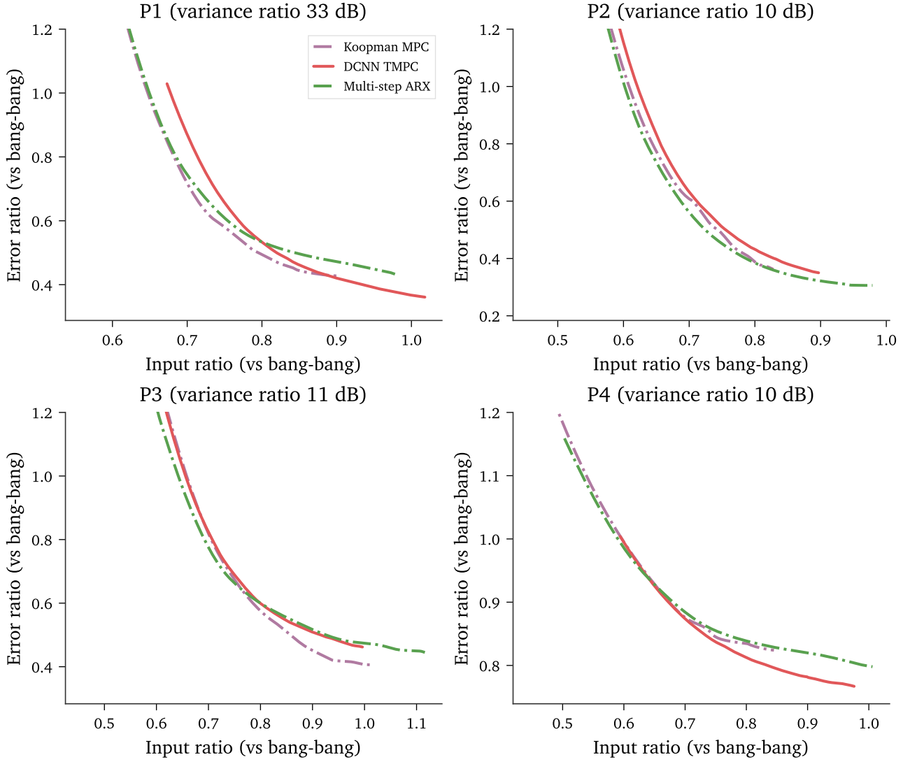
Figure 7.5: Pareto frontiers for three MPC methods across four patients. Lower-left is better.
