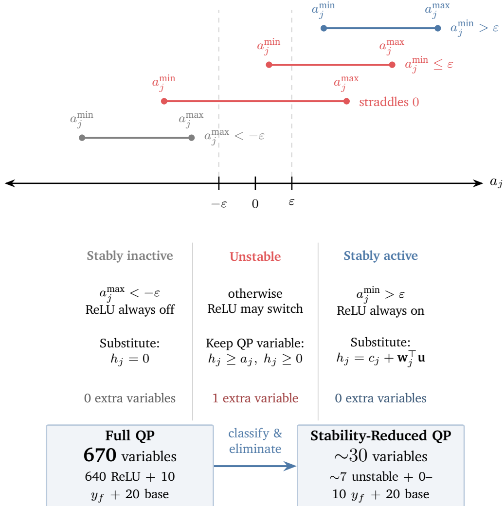
Figure 5.1: Neuron status by pre-activation bounds. Only the \sim 1\% unstable neurons (median 7 of 640 at 50 Hz) retain QP variables, cutting the problem from 670 to \sim 30 variables.
