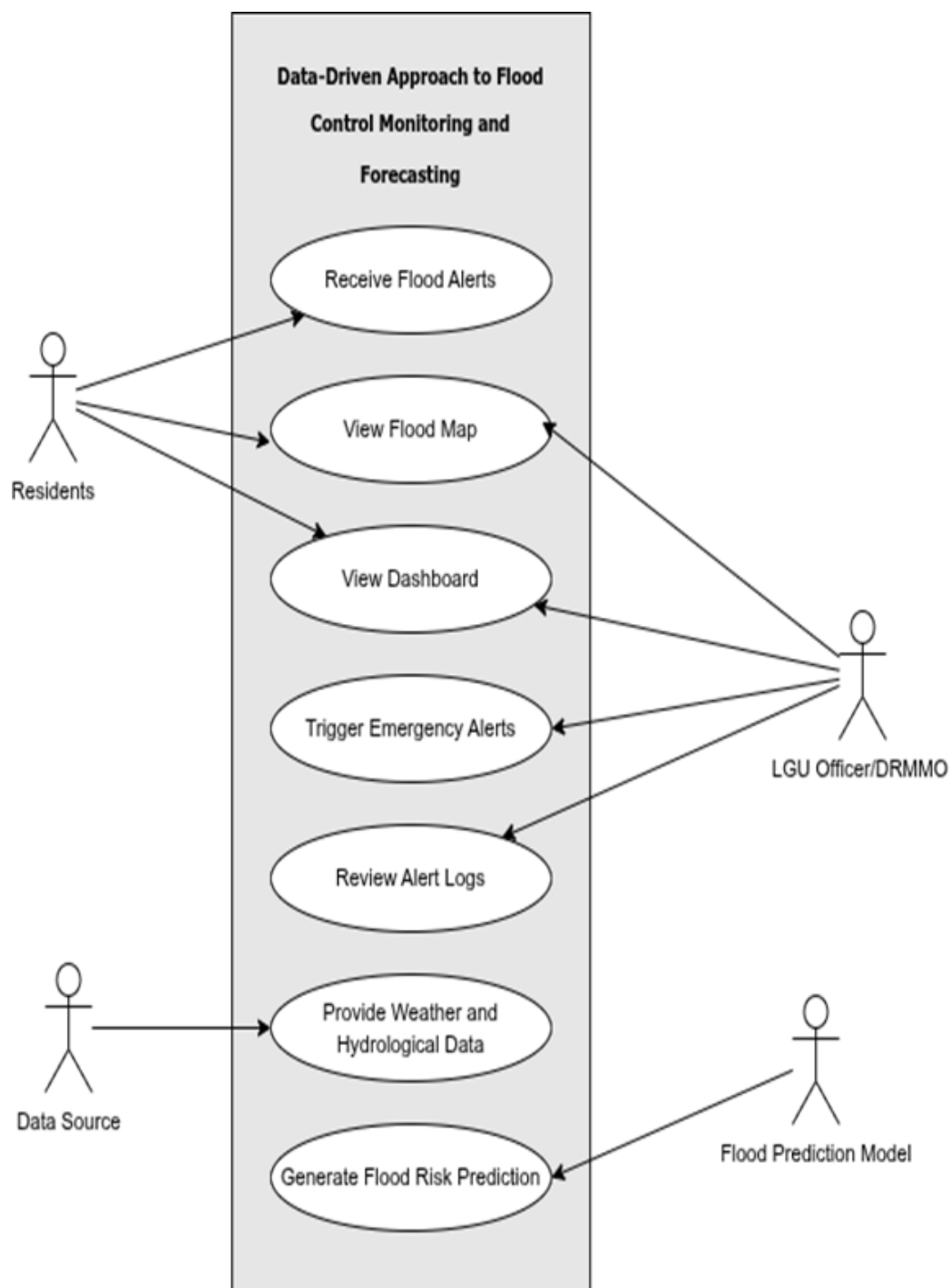
Figure 2.1: Use Case Diagram
