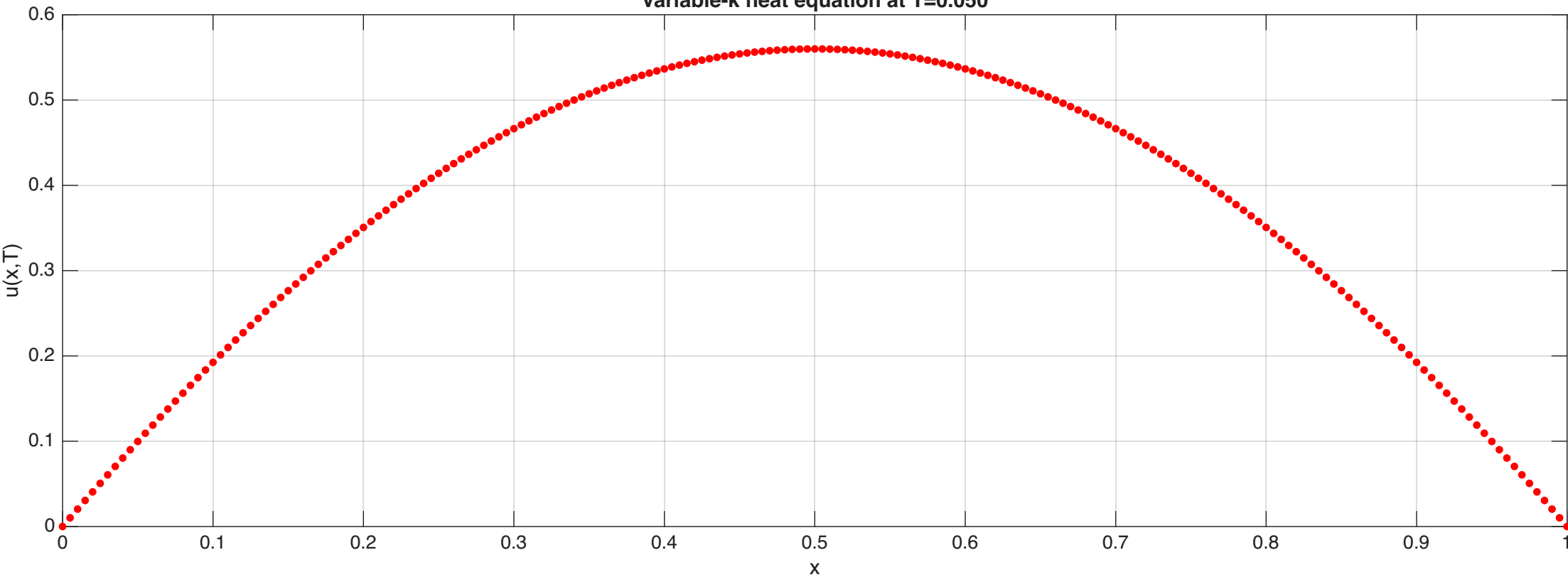
Variable-k heat equation at T=0.050
