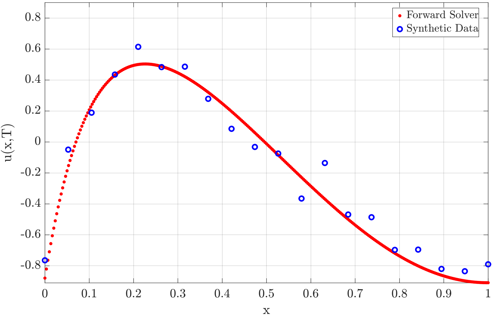
Heat Equation at t=0.0100
