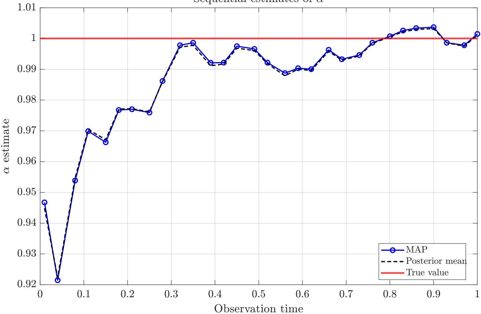
Sequential estimates of \alpha
