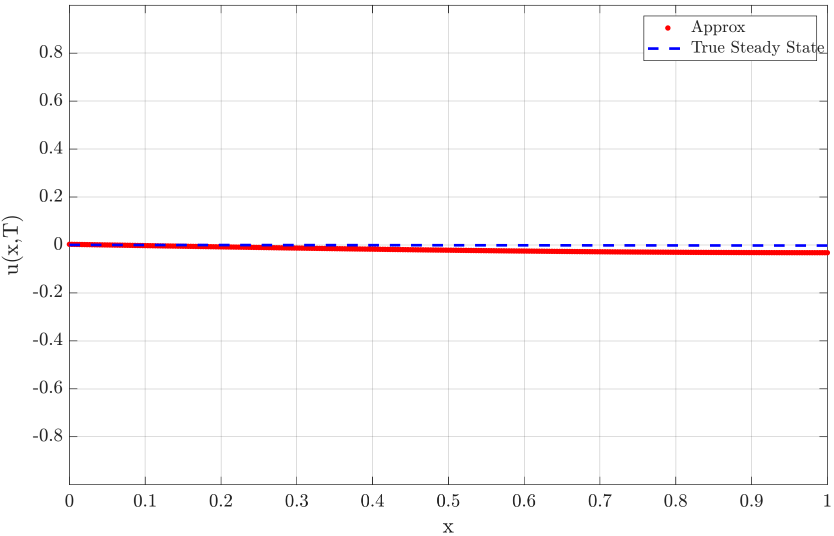
Heat Equation at t=1.0000
