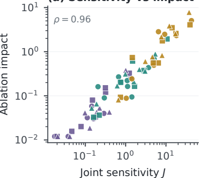
(a) Sensitivity vs impact
