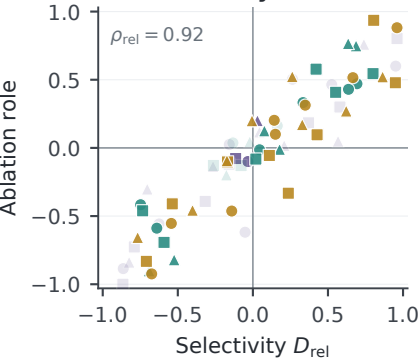
(b) Selectivity vs ablation
