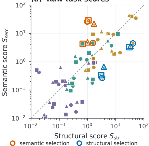
(a) Raw task scores
