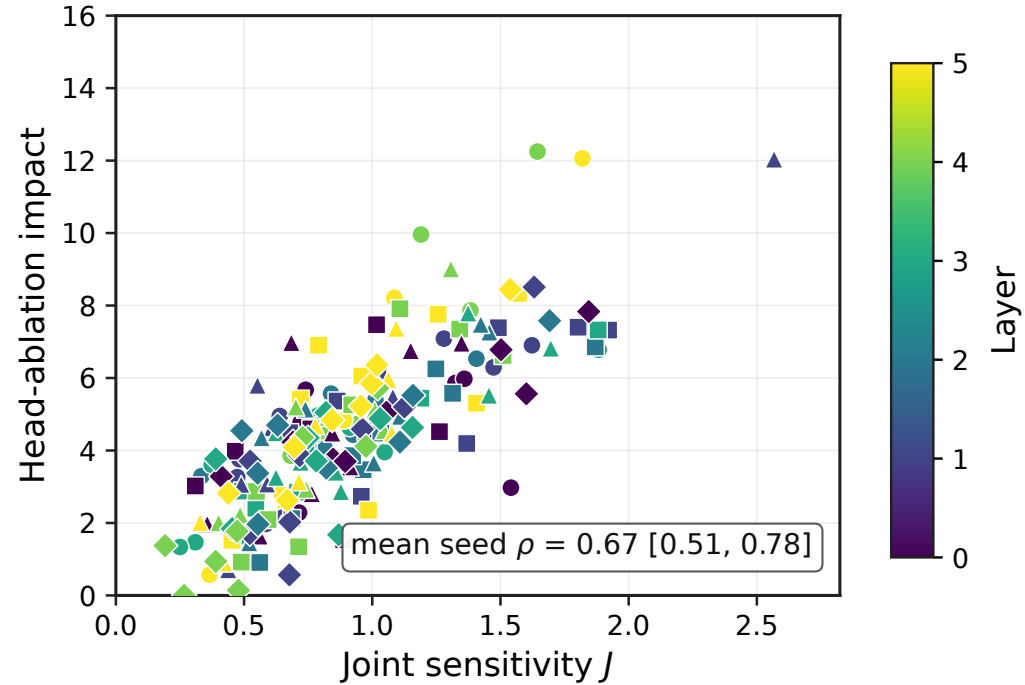
(c) Joint sensitivity and head-ablation impact
