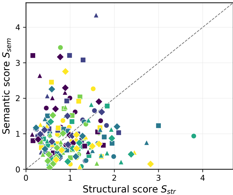
(a) Semantic and structural head scores
