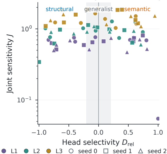
(b) Sensitivity and selectivity
