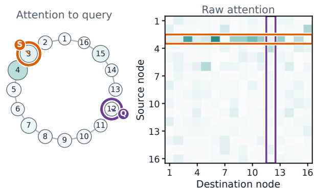
b Structural specialist
