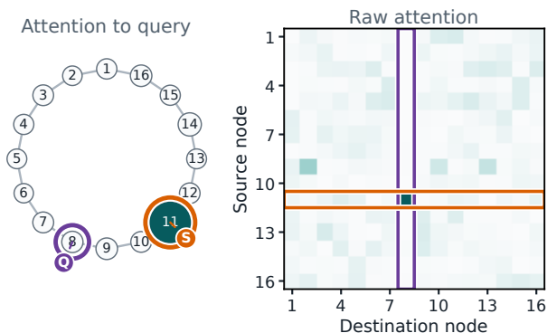
a Semantic specialist
