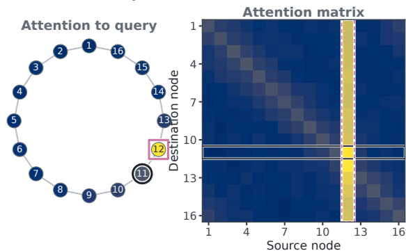
(c) High-/ generalist L2 H4 J = 2.71 D_{\text{rel}} = +0.11
