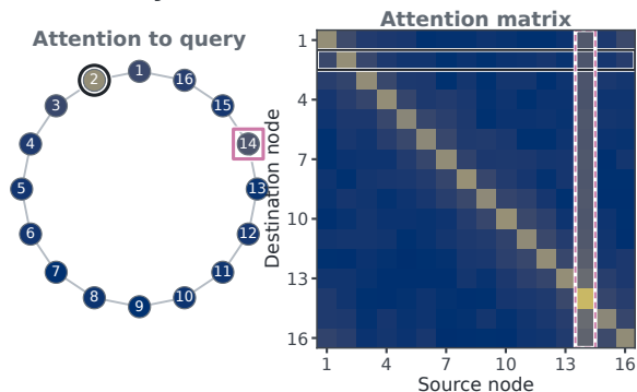
(d) First-layer head L1 H7 J = 0.42 D_{\text{rel}} = +0.71
