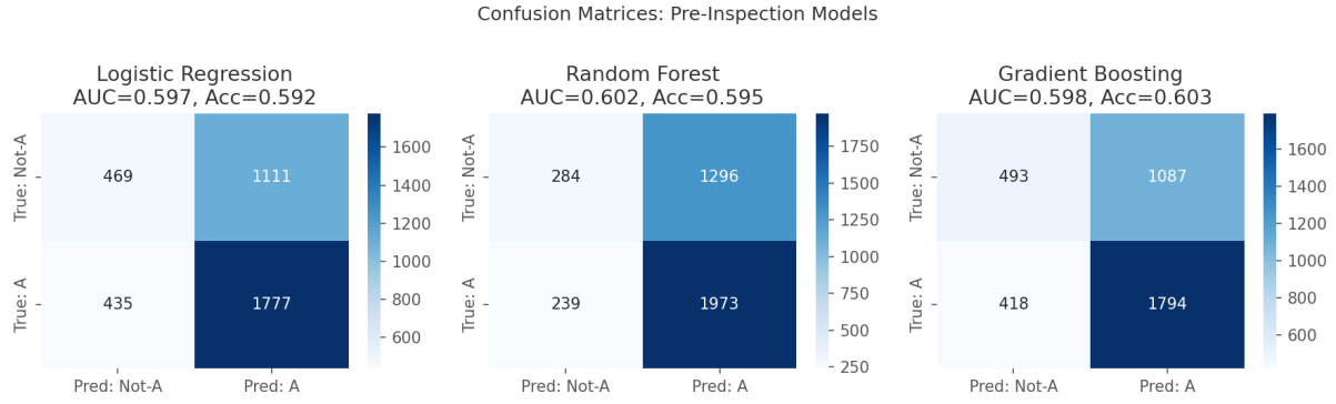
Figure 12: Confusion matrices for the three pre-inspection predictive models. All three models show similar error patterns, consistent with the low AUC.
