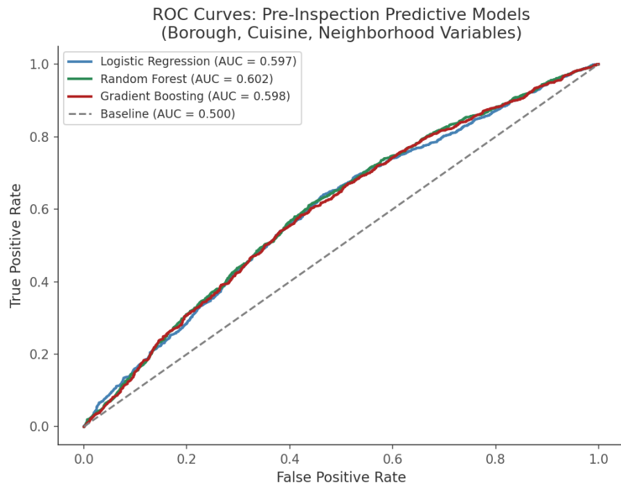
Figure 10: ROC curves for the three pre-inspection predictive models. All three cluster near AUC = 0.60 , slightly above the diagonal (random guessing), confirming that borough, cuisine, and neighborhood variables provide limited predictive power regardless of model choice.
