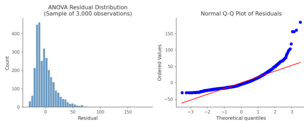
Figure 11: ANOVA residual distribution (left) and normal Q-Q plot (right) for a sample of 3,000 observations. Residuals are clearly right-skewed, violating the normality assumption. This motivates our use of the Kruskal-Wallis test as a non-parametric robustness check ( H = 384.86 , p < 0.001 ), which reaches the same substantive conclusion.
