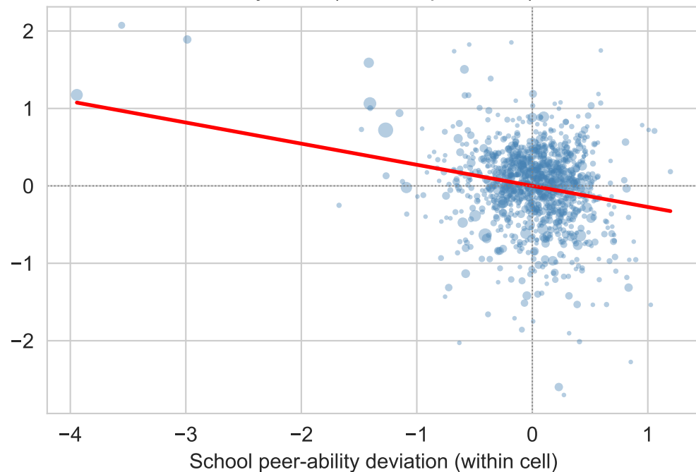
Kenya Y2 ( F=46.8 , \beta=-0.273 )
