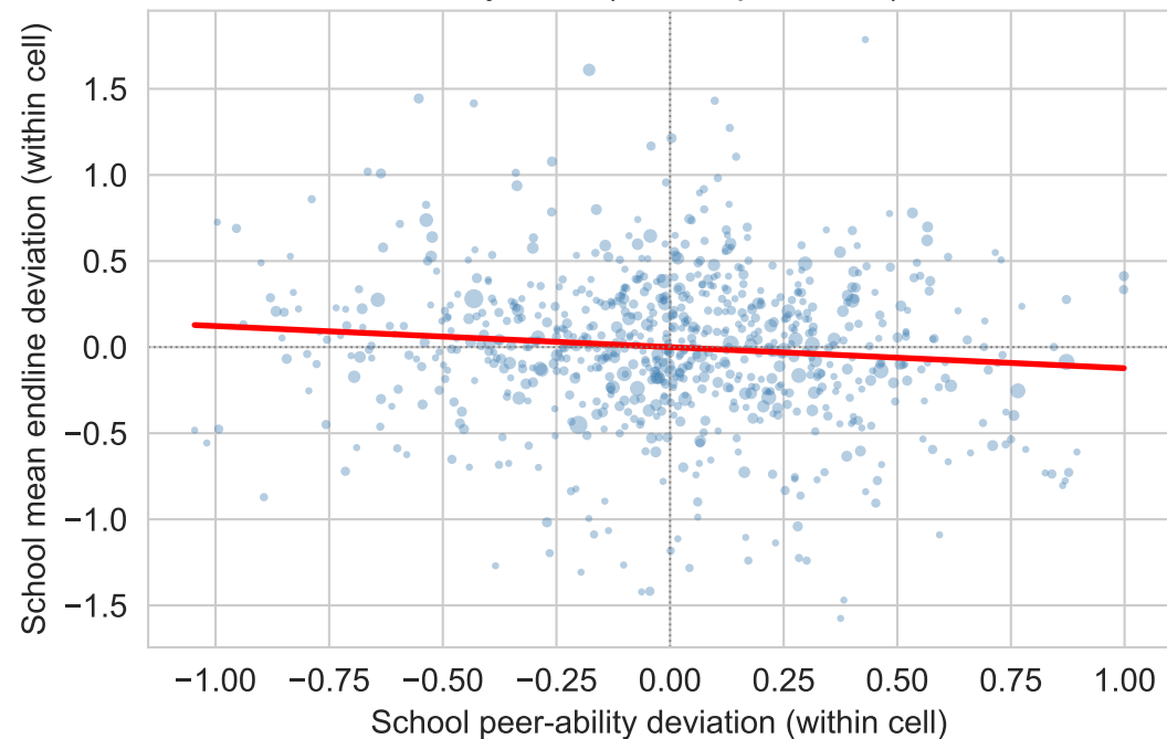
Kenya Y1 ( F=7.7 , \beta=-0.122 )
