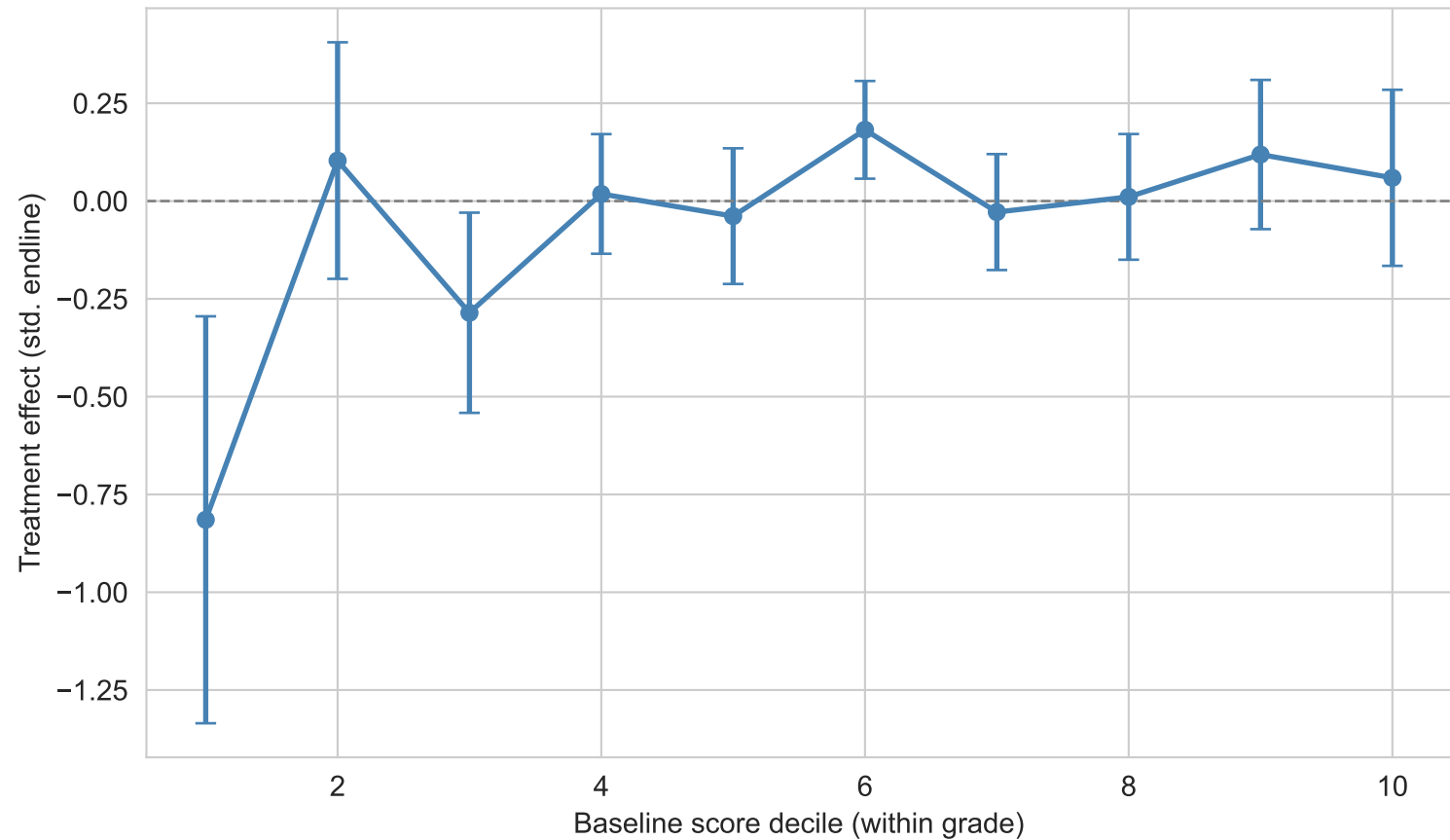
\tau(s) : Treatment effect by baseline ability (Kenya 2019)
