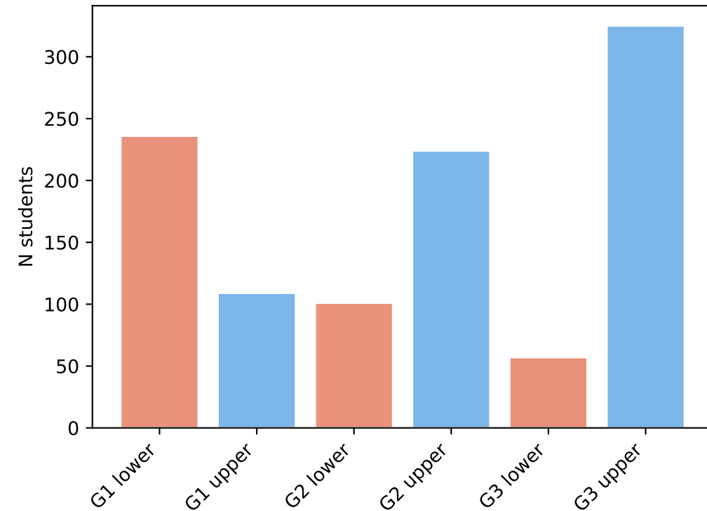
Grade composition at cutoff=36
