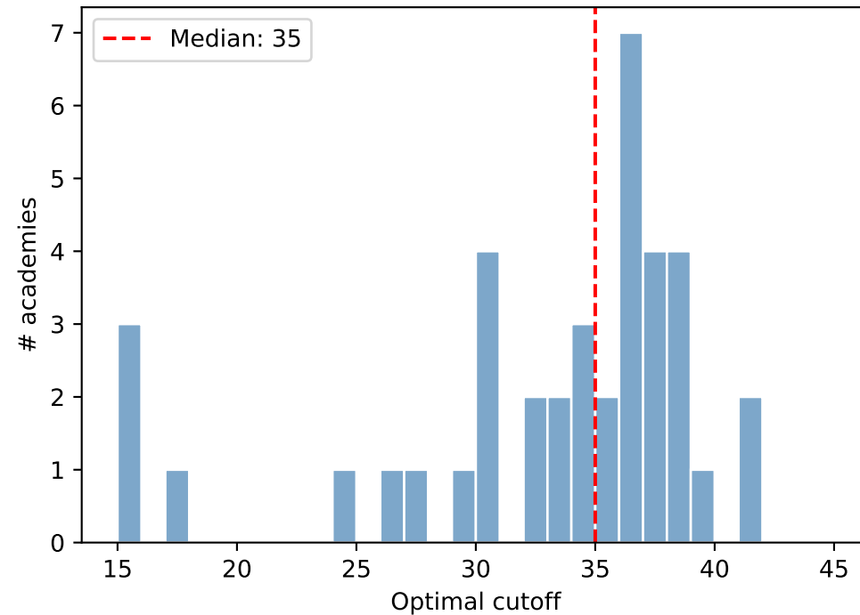
Academy-specific optimal cutoffs
