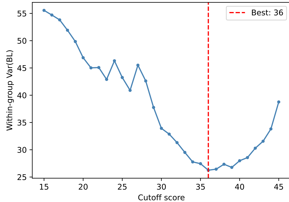
2-group model: optimal cutoff
