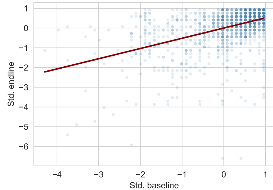
Grade 3 ( R^2=0.226 , N=1564 )
