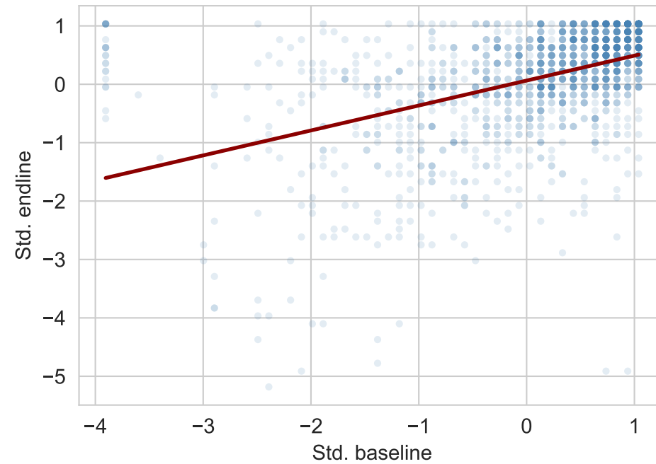
Grade 2 ( R^2=0.205 , N=1618 )
