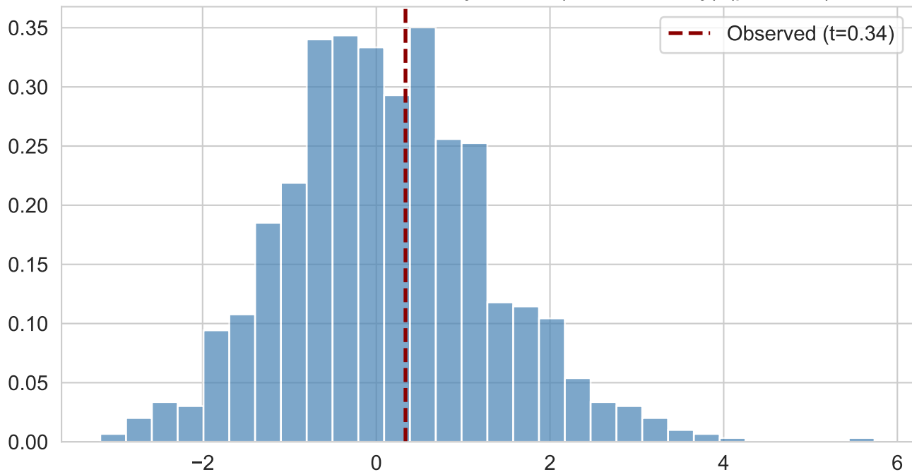
Permutation inference — Kenya 2019 (matched only) ( p=0.779 )
