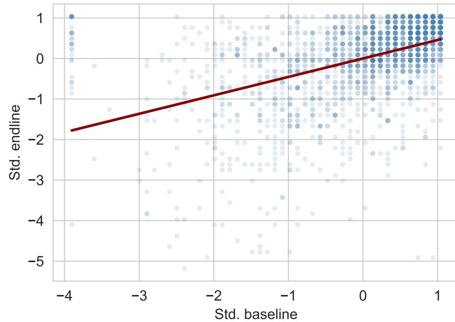
Grade 2 ( R^2=0.208 , N=2227 )
