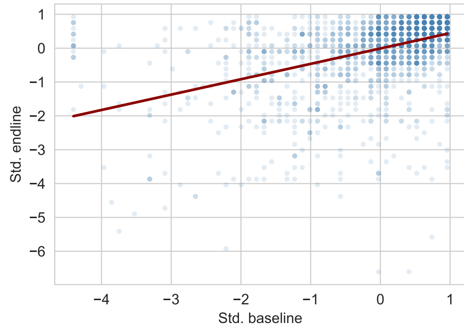
Grade 3 ( R^2=0.205 , N=2180 )
