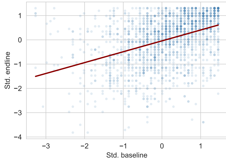
Grade 1 ( R^2=0.169 , N=1936 )
