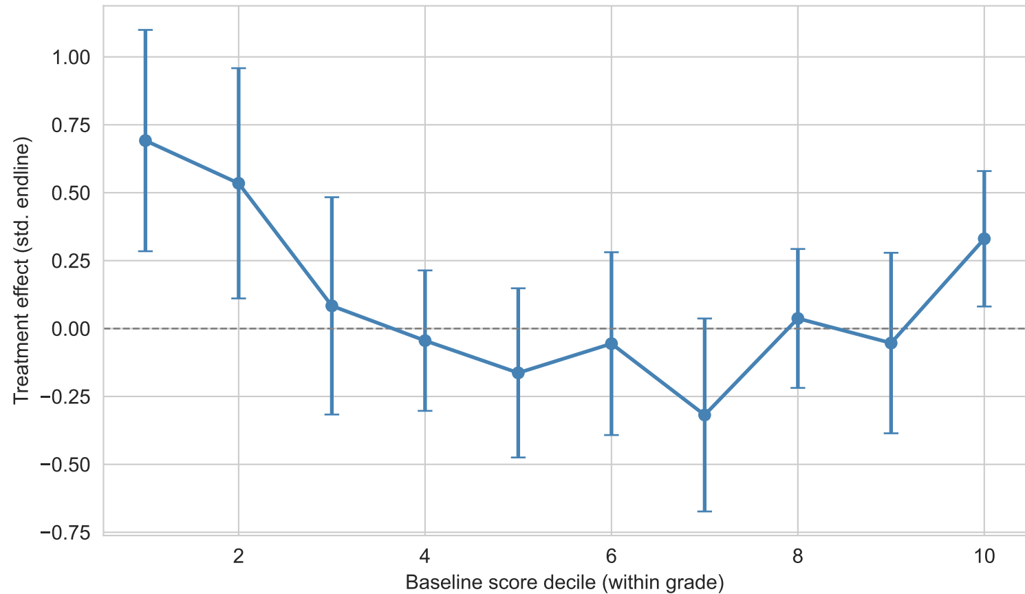
\tau(s) : Treatment effect by baseline ability (Kenya)
