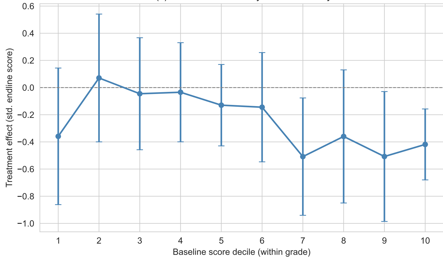
\tau(s) : Treatment effect by baseline ability
