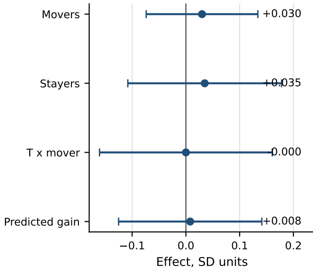
B. Kenya payoff tests
