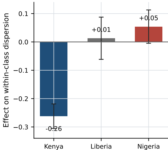
A. Sorting first stage
