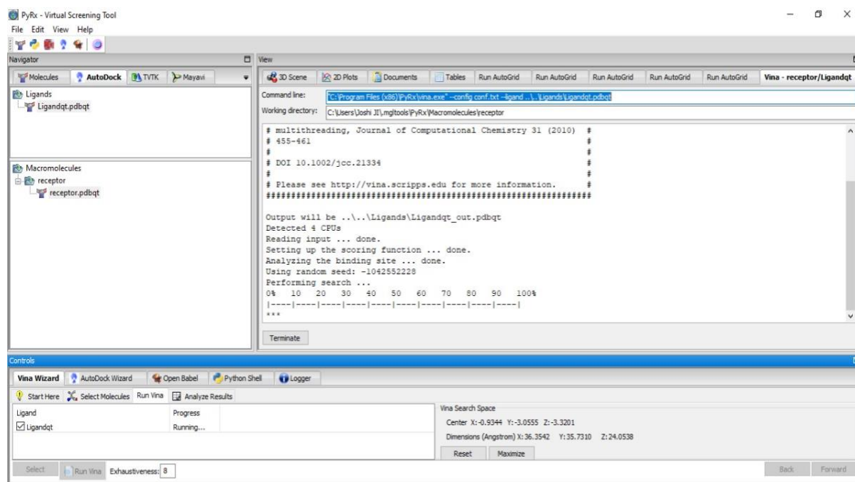
Figure 14: (AutoDock)
