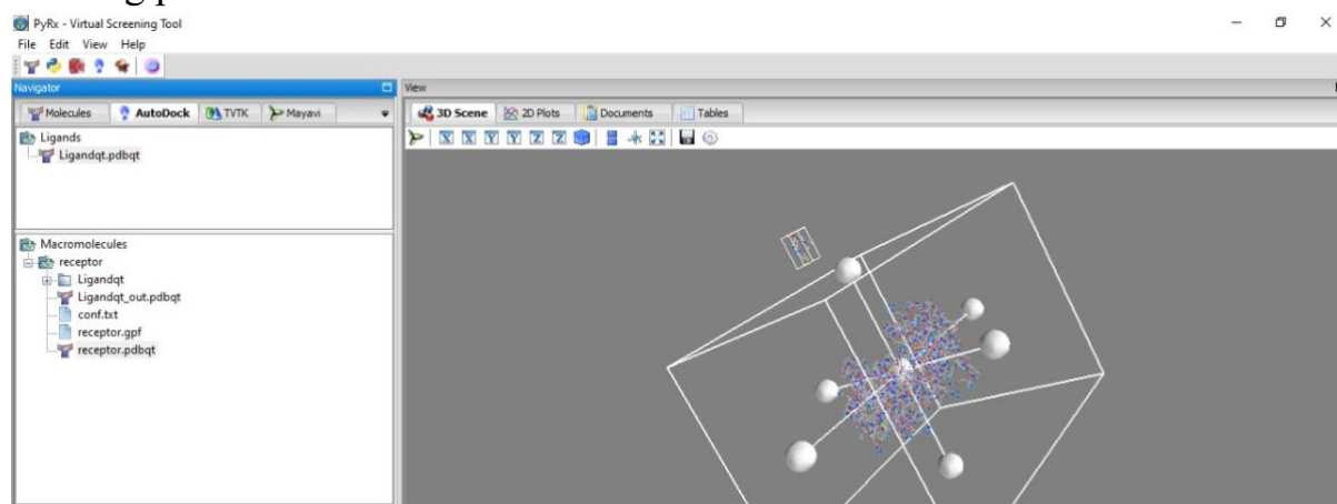
Figure 13: (AutoGrid)
