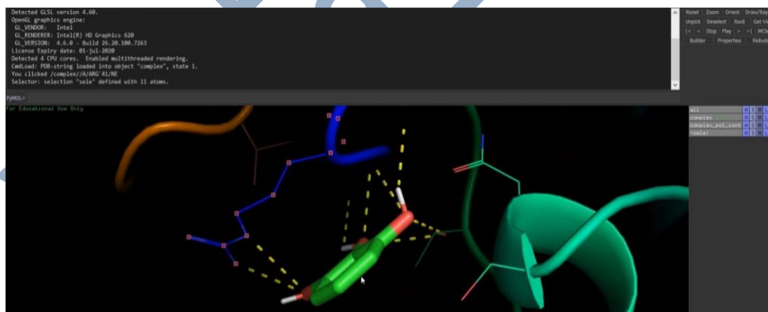
Figure: 17 (hydrogen bonds)
