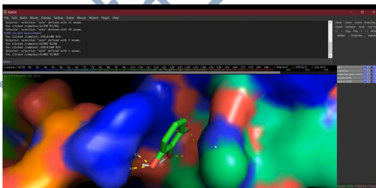
Figure: 18 (molecular surface level format)
