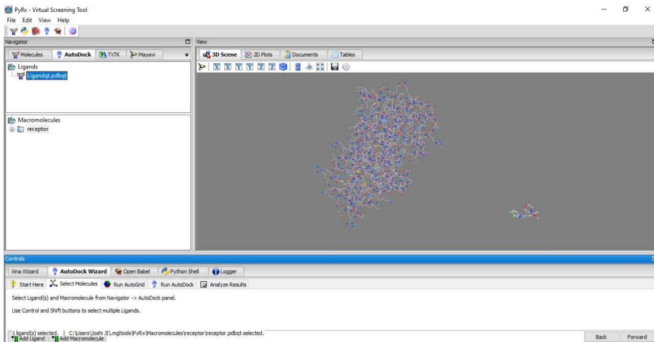
Figure 11: (AutoDock Wizard)
