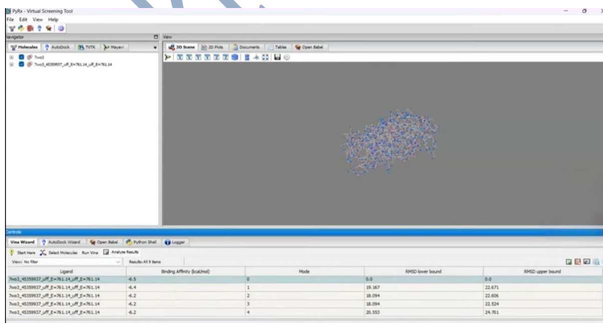
Figure: 15 (AutoDock Results)
